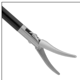
Maryland Extra Fine Dissector, gently curved, double action, ∅ 5mm
